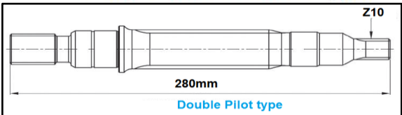
# Drive Shaft-Double Type
