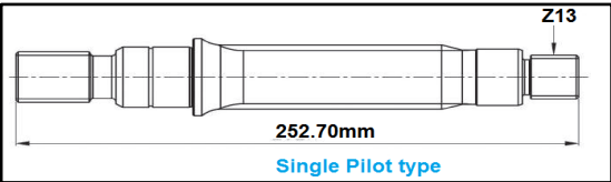
# Drive shaft-Single type
